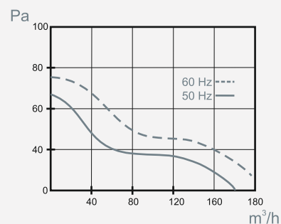
Performance curves
